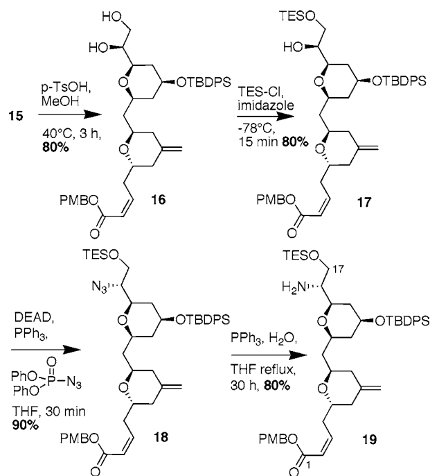
Scheme 4. Completion of the C1–C17 Segment of Phorboxazole B
