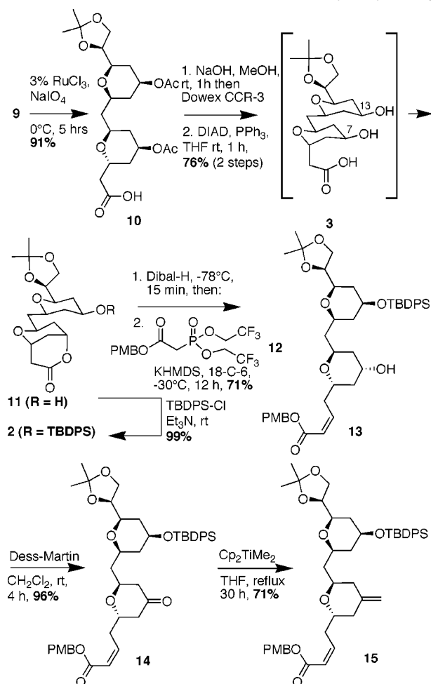
Scheme 3. Differentiation of the C7 and C13 Hydroxyl Groups
