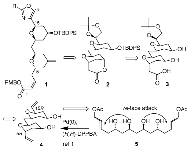
Scheme 1. Retrosynthesis of C1–C17 Segment of Phorboxazole B
