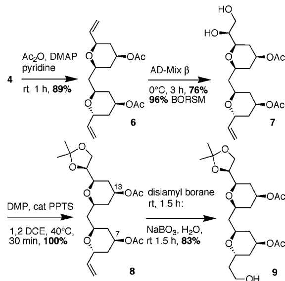
Scheme 2. Differentiation of the C5 and C15 Vinyl Groups
